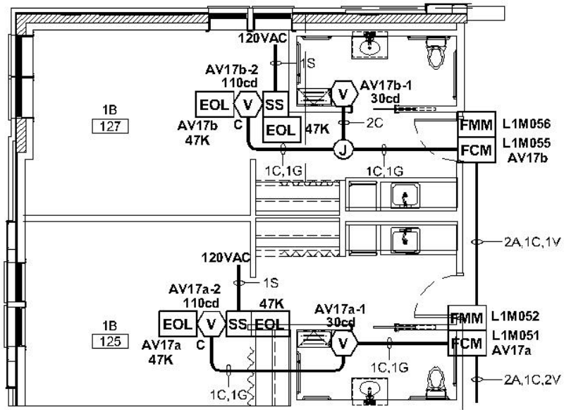
1-BEDROOM TYPICAL with 120VAC SINGLE STATION SMOKE DETECTOR
